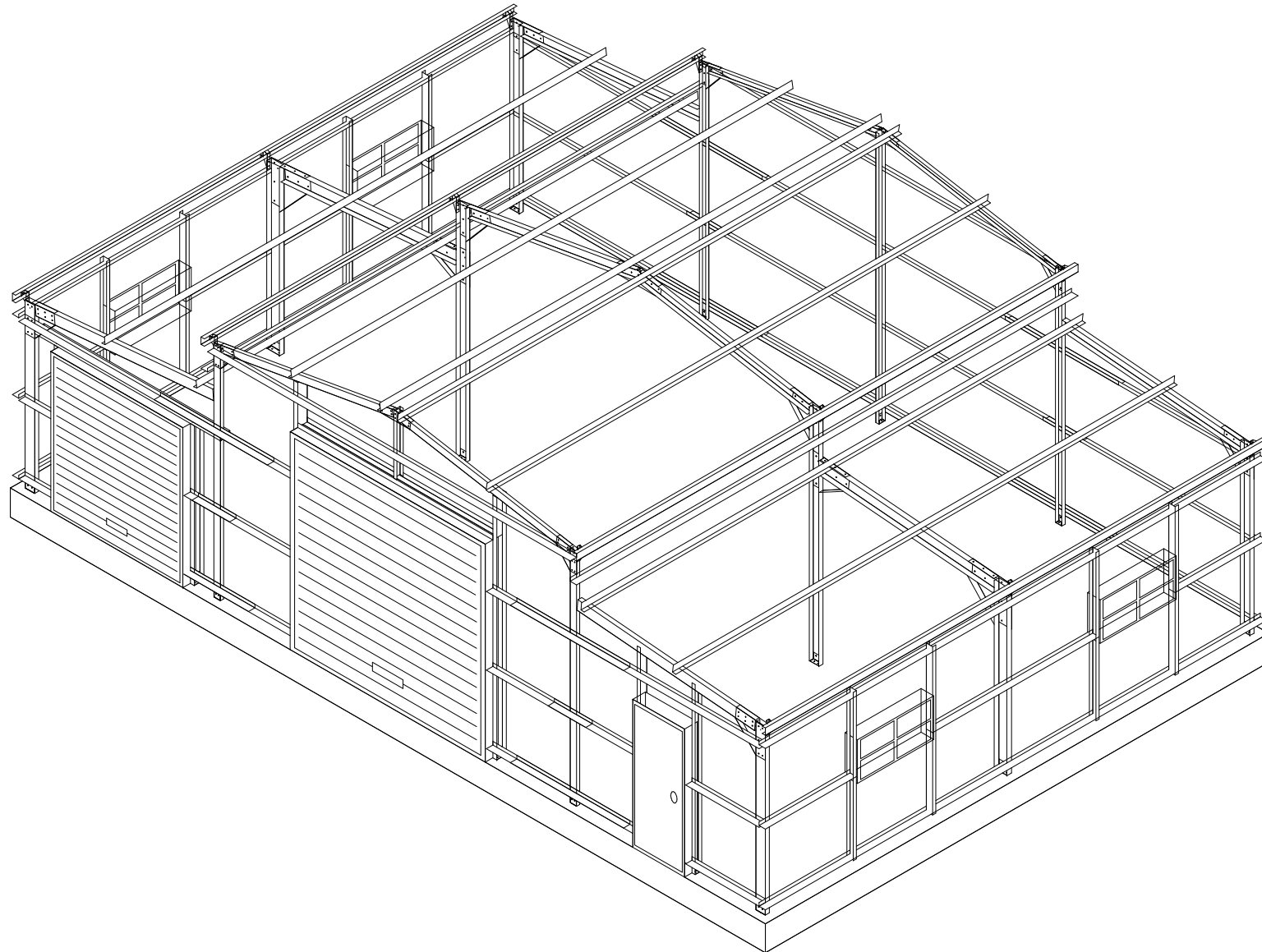
Shed ISO Back Right View (Unclad)
