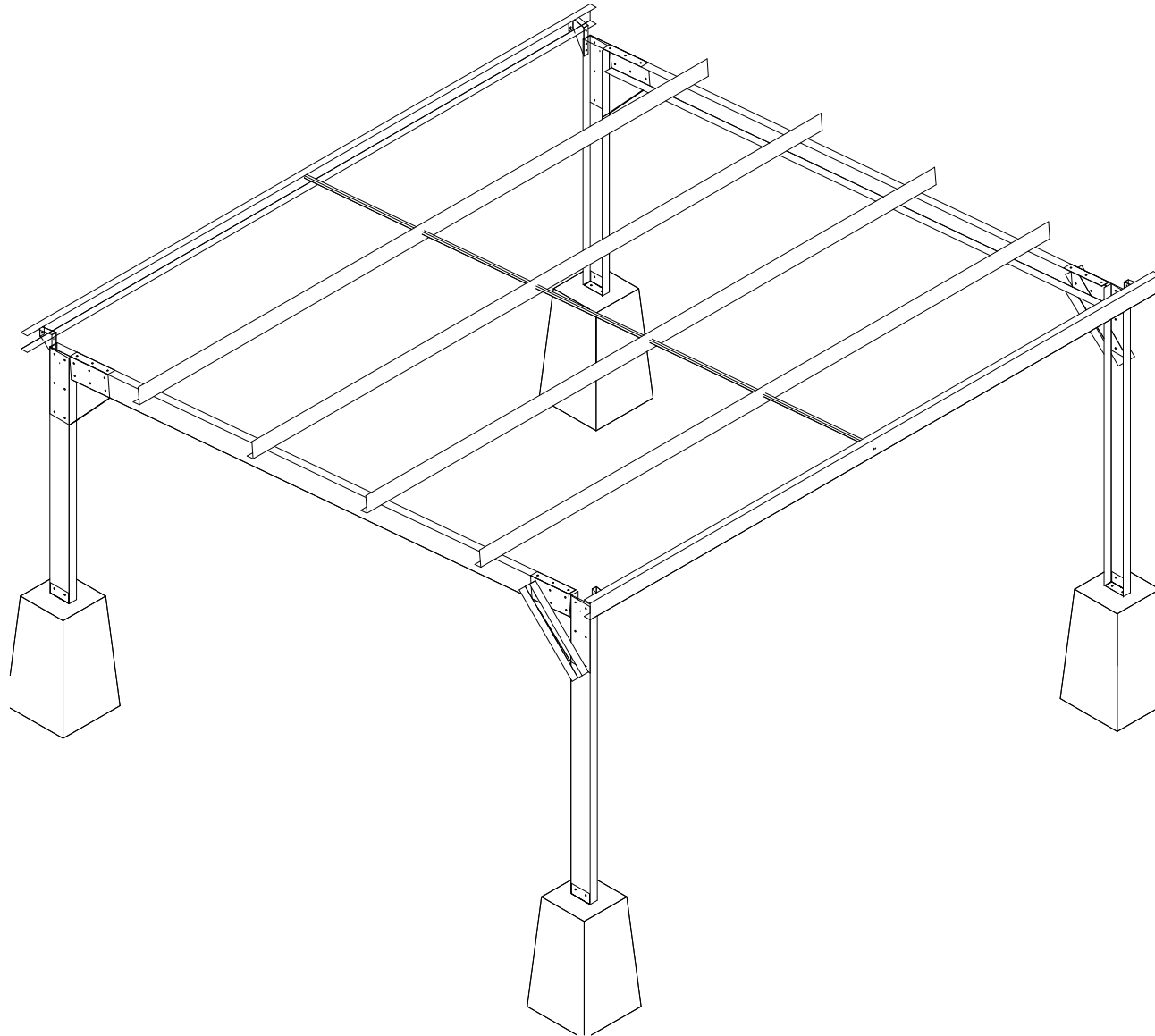
Shed ISO Back Right View (Unclad)
