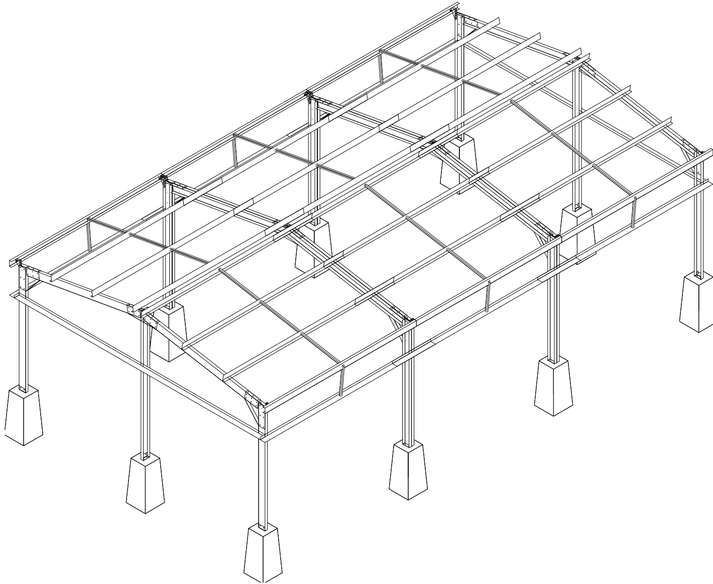
Shed ISO Back Right View (Unclad)
